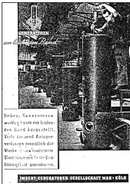
Ill. 85: The Imbert Generator was the most common wood gas generator of the Third Reich, here during its mass production on a conveyor belt in Cologne during 1943. ( Motortechnische Zeitschrift , no. 6/7, 1943, p. 3A.)
