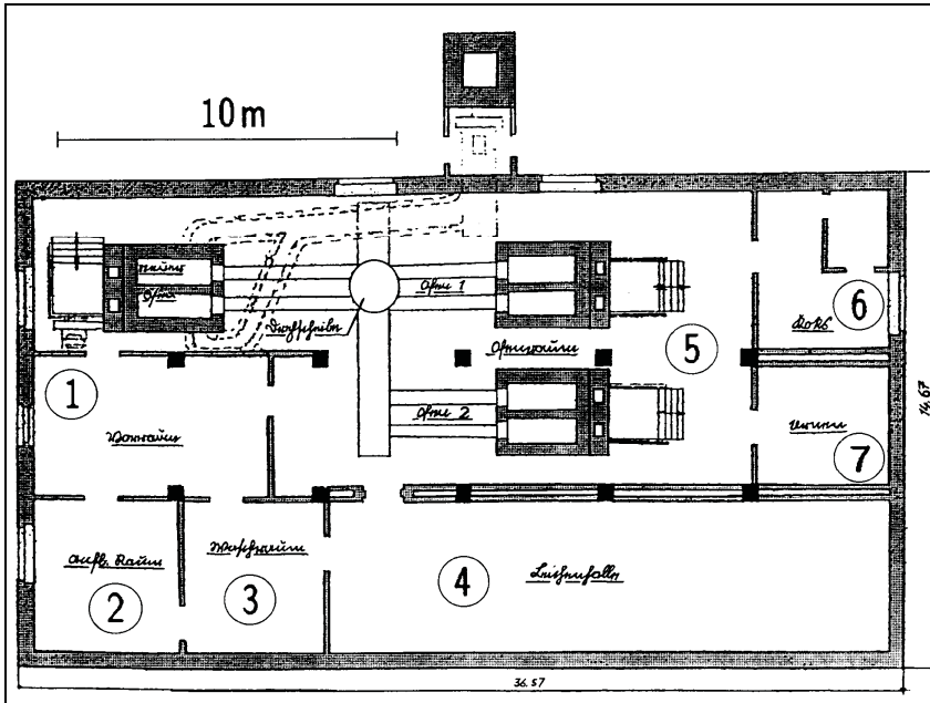
III. 64: Floor plan of Crematory I, Auschwitz main camp, as originally planned.
