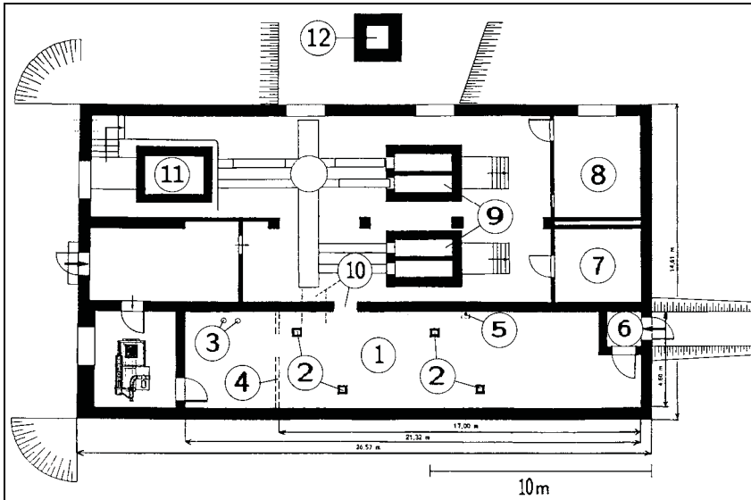
III. 67: Ground plan of Crematory I in main camp as it exists today, following post war alterations. 1: "gas chamber"; 2: hatch for inserting Zyklon B; 3: sewer line for toilets; 4: former dividing wall between morgue and washroom, now removed; 5: ventilation shaft for air raid shelter; 6: air lock to air raid shelter, now called "victims' entrance;" 7: urns; 8: coke; 9: reconstructed oven; 10: opening to oven room at wrong location (original location at dotted lines); 11: remains of old oven; 12: chimney dummy .
