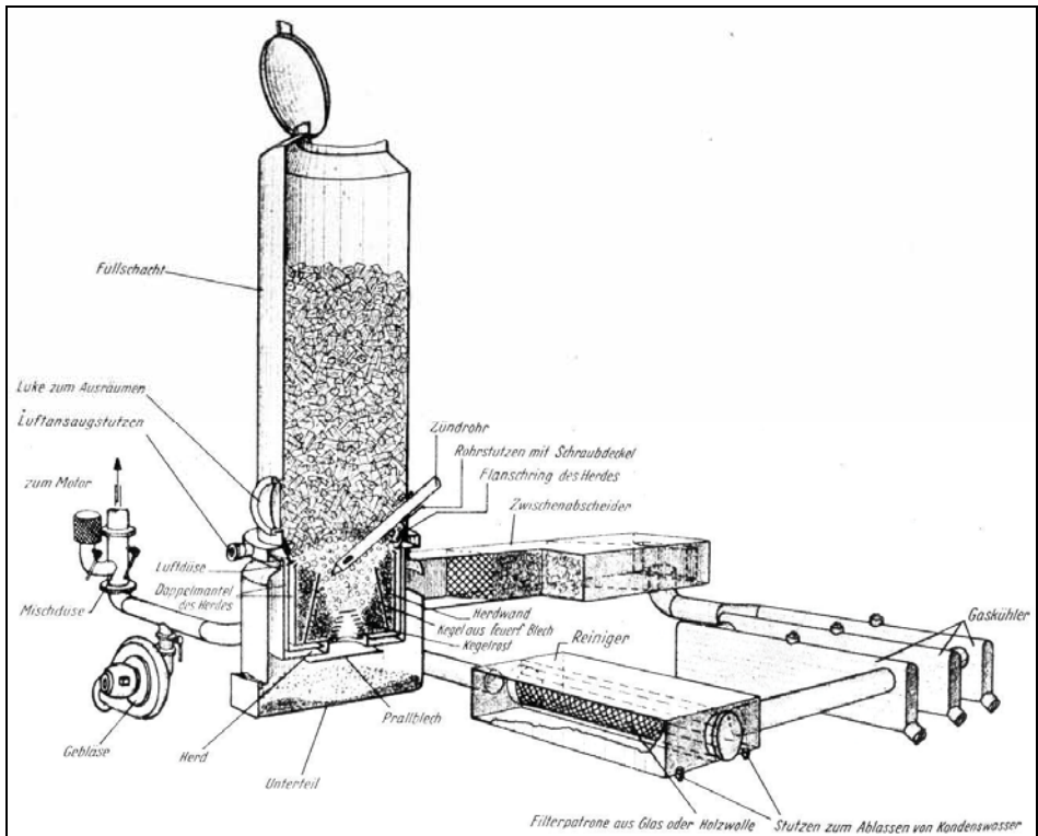
III. 88: Design of an Ostmark Gas Generator.
