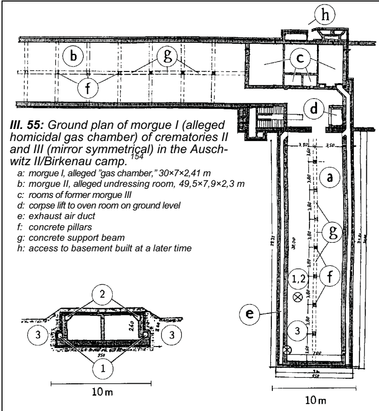
III. 56 (bottom left): Cross section through morgue #1 (alleged homicidal gas chamber) of crematories II and III (mirror symmetrical) in Auschwitz-Birkenau. 154 1: exhaust air duct; 2: fresh air duct; 3: soil
