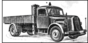
III. 86: The Austro-Fiat 4 D 90 A, manufactured with wood burning gas generator.
