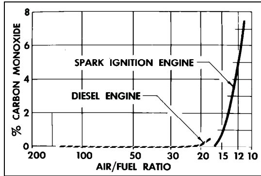
III. 83: Carbon monoxide content of exhaust gases from spark engines and diesel engines as a function of engine load (air/fuel ratio)
